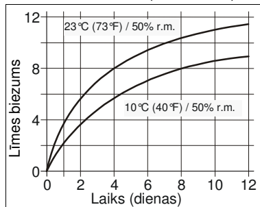
Att. 1: Cietēšanas process SikaTack®-Drive (New Formulation) līmei
